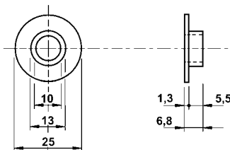
610054 Bushing
