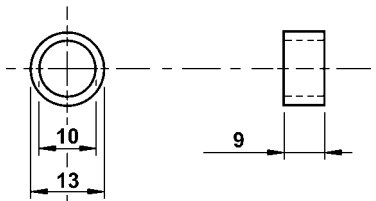
610053 Bushing
