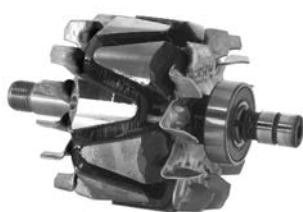
137331 Rotor
