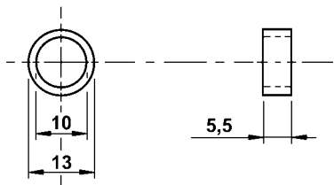
610050 Bushing
