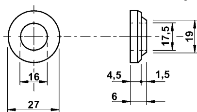
610057 Rubber Bushing
