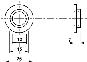
610188 Bushing
