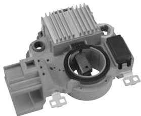
331005 Regulator
