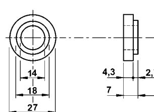
610058 Rubber Bushing
