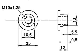
610052 Bushing
