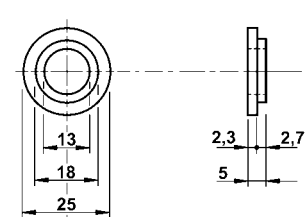
610059 Rubber Bushing
