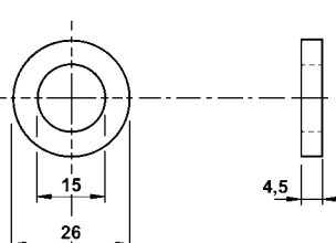
610056 Rubber Bushing
