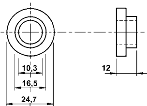
610060 Steel bush
