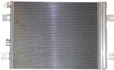
260446 Condenser Replacing: 92100-JD51A, 92100-JD500 Servicing: Nissan Dryer w/o A: 405.00 B: 643.00 C: 20.00 mm
