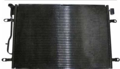
260508 Condenser Replacing: 8E0260403D, 8E0260401D Servicing: Audi Dryer w/o A: 400.00 B: 605.00 C: 20.00 mm
