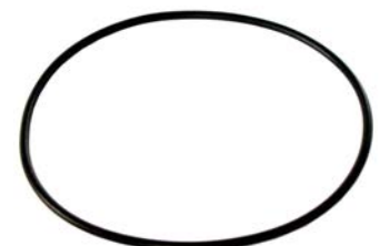
252641 O-ring ID 102.00, Thickness 3.00, Material Rubber
