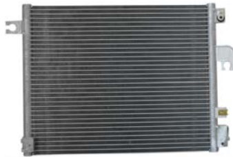
260398 Condenser Replacing: 9760605500 Servicing: Hyundai Dryer w/o A: 350.00 B: 445.00 C: 18.00 mm
