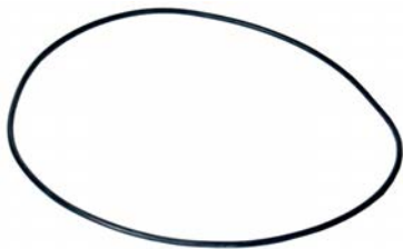
251173 O-ring ID 120.00, Thickness 2.00, Material Nioprene
