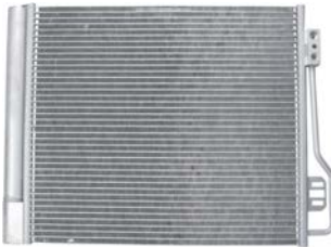
260426 Condenser Replacing: 4515000154, 4515000054 Servicing: Smart (MCC) Dryer w/ A: 385.00 B: 448.00 C: 20.00 mm
