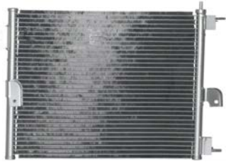
260397 Condenser Replacing: 9760602200, 9760602000 Servicing: Hyundai Dryer w/o A: 345.00 B: 450.00 C: 22.00 mm
