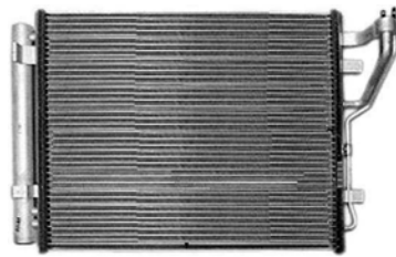
260403 Condenser Replacing: 976062L600, 976062H600 Servicing: Hyundai Dryer w/ A: 398.00 B: 480.00 C: 20.00 mm
