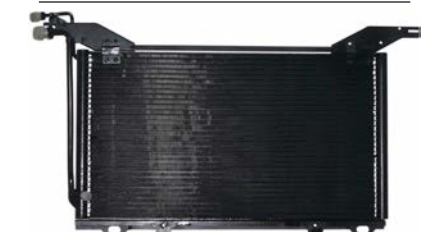
260079 Condenser Replacing: A2108300770, A2108300370 Servicing: Mercedes-Benz Dryer w/o A: 329.00 B: 617.00 C: 25.00 mm
