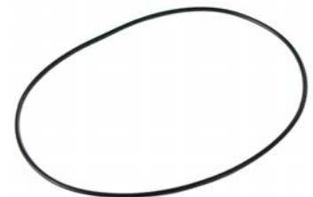
252482 O-ring ID 104.00, Thickness 2.00, Material Nioprene
