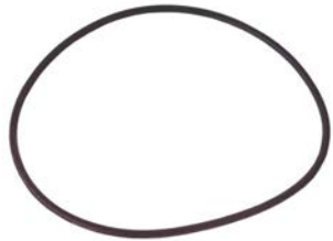
250186 O-ring ID 114.00, Thickness 3.00, Material Nioprene
