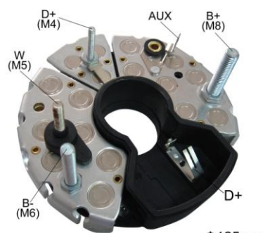
Φ125mm
