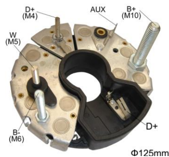
Φ125mm
