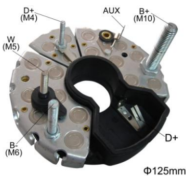
Φ125mm
